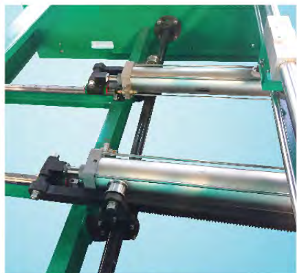
气缸 + 同步齿轮齿条加压 Pressurize by cylinder + synchronous gear rack
